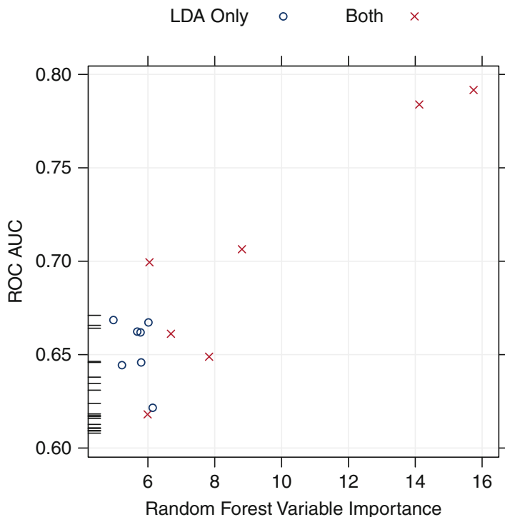
Fig. 19.7: A comparison of two methods for determining variable importance. The random forest values correspond to models with 7 predictors while the ROC values are based on the top 35 predictors (i.e., the best subset for LDA). The values are averaged across the 50 resamples. The “LDA Only” values are predictors that were in the final LDA model but not the random forest model. The hash marks, not the y -axis, are for LDA predictors that were not selected in any of the 50 resampled random forest models
