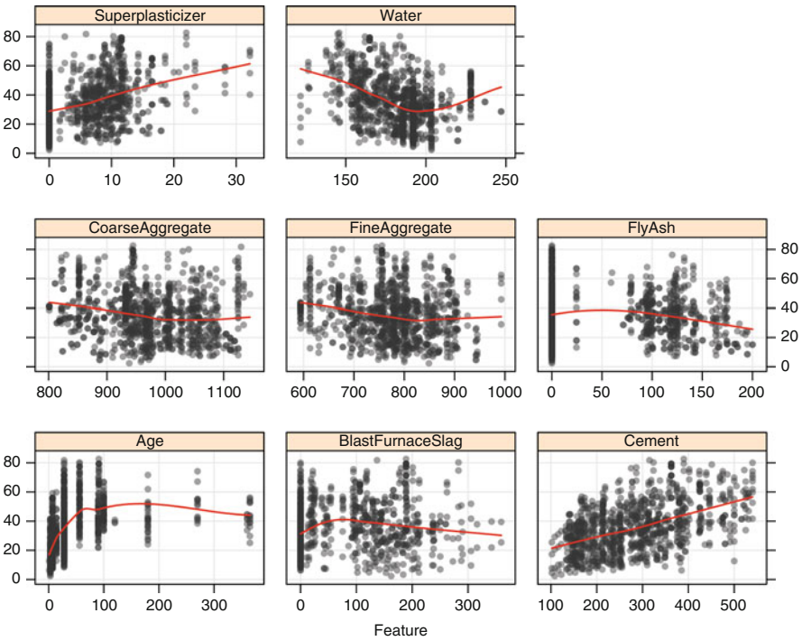
Fig. 10.1: Scatter plots of the concrete predictors versus the compressive strength
